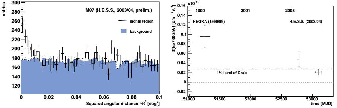
Figure 1. Left: Distribution of ON-source events (solid histogram) and normalized OFF-source events (filled histogram) vs. the squared angular distance \Delta\Theta^2 . Right: The integral photon flux above a threshold of 730 GeV assuming of a power-law energy spectrum with a photon index of \Gamma = 2.9 (as reported by HEGRA [10]). The recent H.E.S.S. measurement in 2004 is not compatible with the HEGRA flux which indicates variability. However, additional systematic uncertainties between the different experiments need to be taken into account. The 1% flux level of the Crab Nebula is also indicated.
