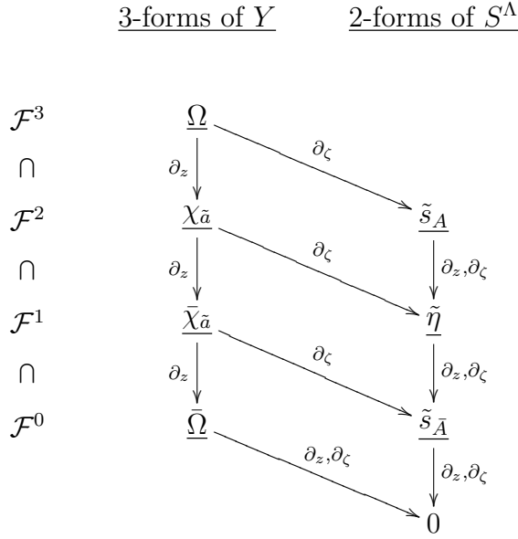
Figure 6.1: Variation of Hodge structure of H^3_-(Y, S^A) .
